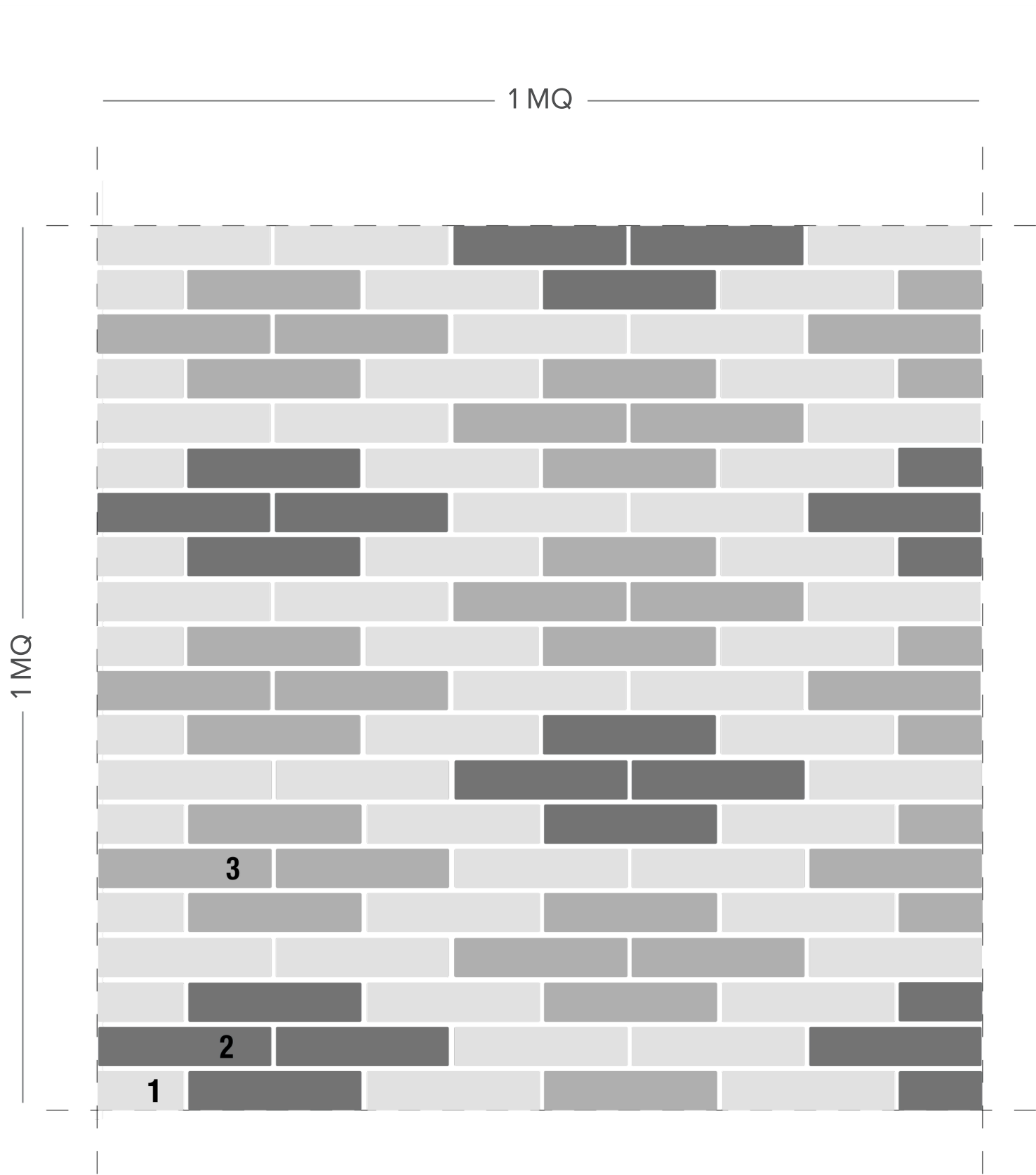
LAYOUT LC32
